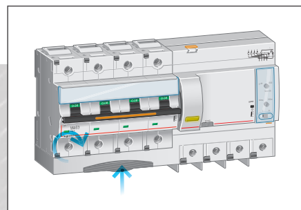
3 TIGHTEN THE TERMINALS and fit the terminal shield
