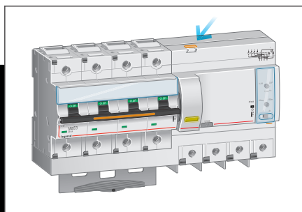
2 LOCK THE COMBINATION TOGETHER
