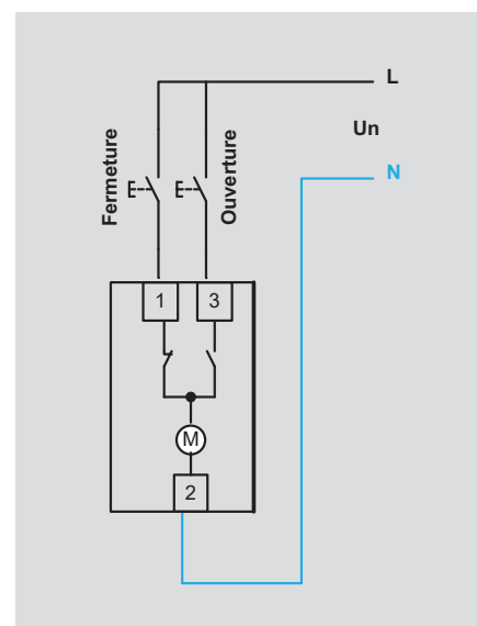
Standard motor
