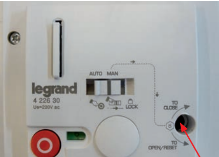
Hole for manual opening/closing
