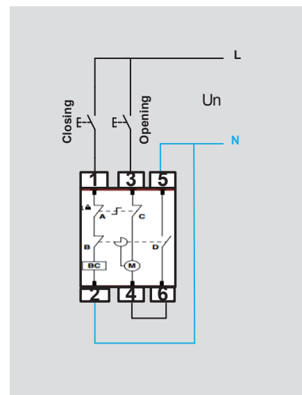
Configured motor
