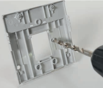
Drill the 8 mm diameter hole.
